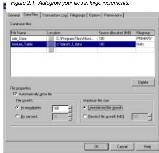
Figure 2.1: Autogrow your files in large increments.
