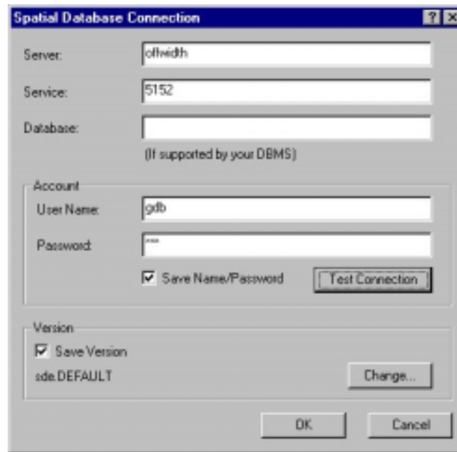
Figure 5.1: Connecting to a server through ArcCatalog
