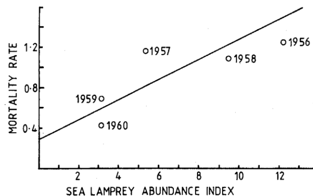
Fig. 8.3 Instantaneous annual mortality of lake trout, Salvelinus namaycush , in relation to an index of sea lamprey, Petromyzon marinus , abundance in Lake Ontario during the 1950s. Redrawn with permission from Christie (1974).
