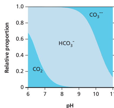
Distribution of inorganic carbon species in water as a function of pH.
