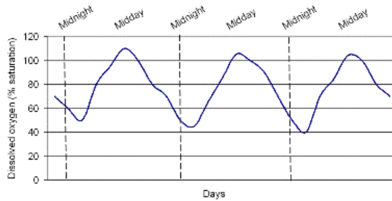
Example patterns in dissolved oxygen levels for a lowland river
