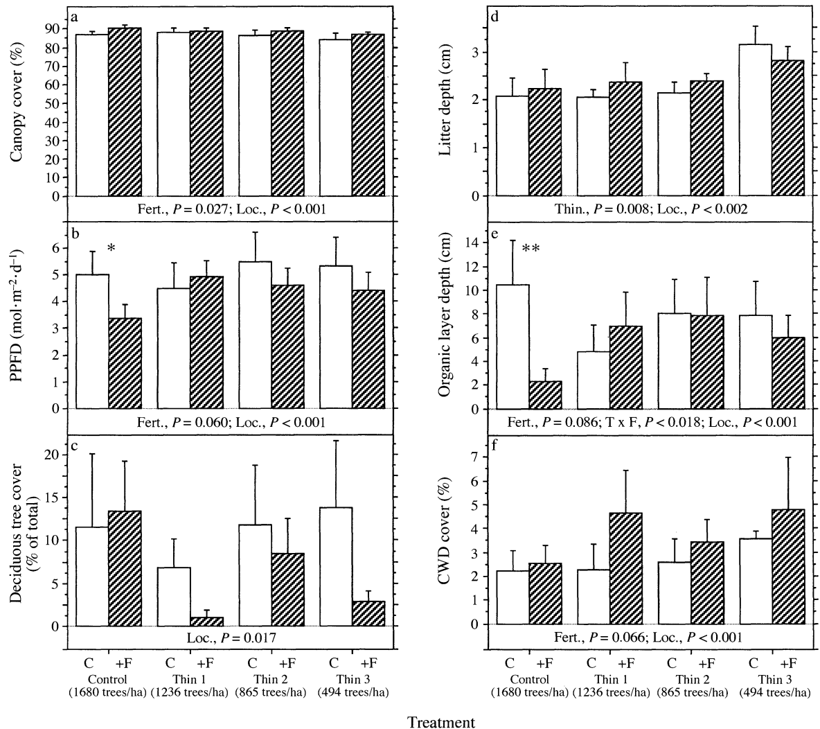
FIG. 1. Responses (means and 1 SE) of overstory canopy and edaphic characteristics to thinning and fertilization in 21–27 yr old Douglas-fir plantations. Hatched bars indicate stands repeatedly fertilized with urea (see Table 1 for details of addition rates). Asterisks indicate significance of a posteriori contrasts between control (C) vs. fertilization (+F) treatments within a given thinning level: * P < 0.05 , ** P < 0.01 . Probability values are listed for significance of thinning (Thin.), fertilization (Fert.), location (Loc.), and thinning \times fertilization interaction (T \times F) terms for each variable.
