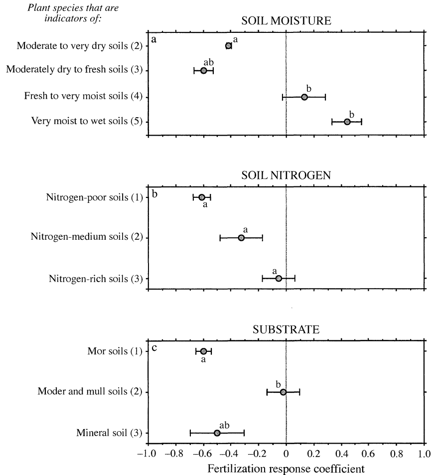
FIG. 6. Differential responses (means \pm 1 SE) of species groups based on soil indicator values given by Klinka et al. (1989). Coefficients give the expected proportional change in cover given an increase in one "unit" of thinning or fertilization (see Methods: Statistical analysis ). Means with the same lowercase letter are not significantly different at P < 0.05 using a posteriori contrasts between groups.
