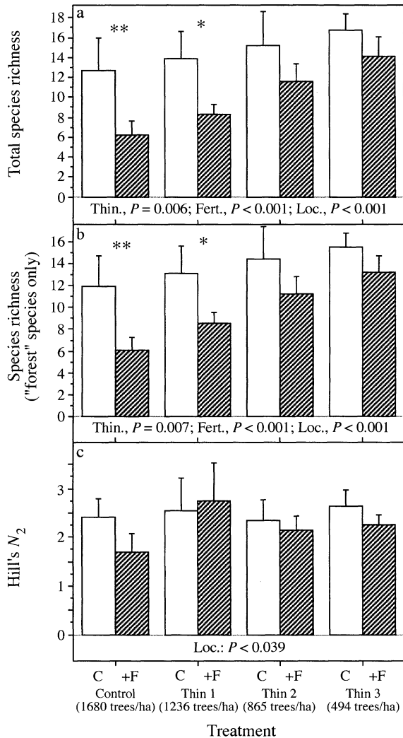
FIG. 3. Effects (means and 1 SE) of thinning and fertilization treatments on vascular-plant diversity quantified as (a) total number of species within sampled 62.5-m 2 subplots; (b) total number of "forest" species within sampled 62.5-m 2 subplots; (c) Hill's N_2 diversity index (all species), calculated as 1/\sum(p_i^2) , where p_i is the proportional cover of species i in the sample unit (Hill 1973). Asterisks indicate significance of a posteriori contrasts between control (C) vs. fertilization treatments (+F): * P < 0.05 ; ** P < 0.01 . Probability values are listed for significance of thinning (Thin.), fertilization (Fert.), location (Loc.), and thinning \times fertilization interactions (T \times F) terms for each variable.
