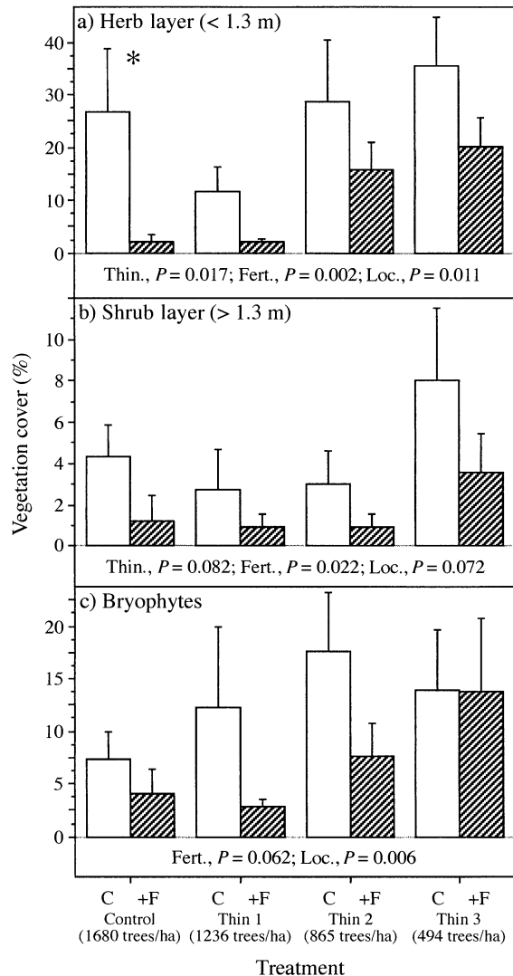
FIG. 2. Responses (means and 1 SE) of understory vegetation cover to thinning and fertilization treatments. Herb-layer vegetation included individuals of all species reaching a maximal height of <1.3 m within sampled quadrats. Shrub-layer vegetation included all species attaining heights >1.3 m. Bryophytes include all species of mosses and liverworts inhabiting soil, litter, or woody debris substrates but exclude epiphytes. Asterisks indicate significance of a posteriori contrasts between control (C) vs. fertilization (+F) treatments: * P < 0.05 . Probability values are listed for significance of thinning (Thin.), fertilization (Fert.), location (Loc.), and thinning \times fertilization interactions (T \times F) terms for each variable.
