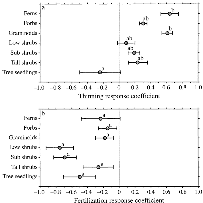
FIG. 5. Differential responses (means \pm 1 SE) of plant life-forms to thinning and fertilization. Coefficients give the expected proportional change in cover given an increase in one "unit" of thinning or fertilization (see Methods: Statistical analysis ). Means with the same lower-case letter are not significantly different at P < 0.05 using a posteriori contrasts between groups.
