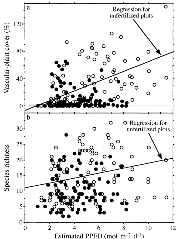
FIG. 7. Relationships between understory light levels (estimated as the annual mean of daily photon flux, using hemispherical photograph analysis) and (a) understory vegetation cover (herb plus shrub layers) and (b) vascular-plant species richness. Solid symbols are fertilized plots; open symbols are unfertilized plots.
