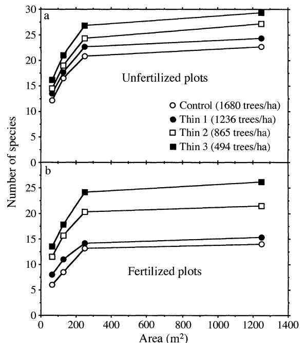
FIG. 4. Species-area curves within each thinning and fertilization treatment combination. Each curve represents the mean across six study locations within a given treatment.
