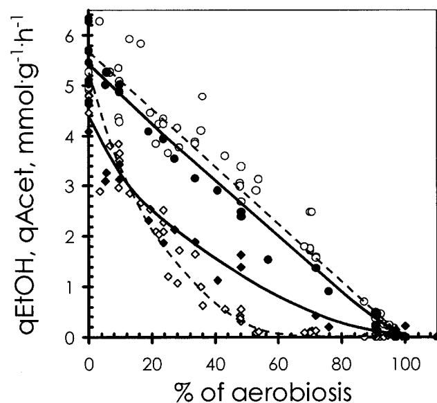
FIG. 2. Effect of the oxygen supply rate on the formation rates of acetate (circles) and ethanol (diamonds) of the wild-type (open symbols) and \Delta arcA (filled symbols) strains. Data for the wild-type strain are derived from reference 1.
