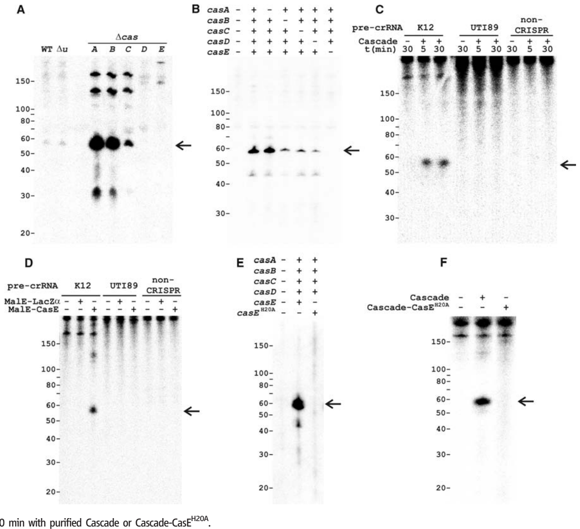
Fig. 2. Cascade cleaves CRISPR RNA precursors into small RNAs of ~57 nucleotides (marked by arrows). (A) Northern analysis of total RNA of WT E. coli K12 (WT), a non- cas gene knockout ( \Delta u , uidA , \beta -glucuronidase), and Cascade gene knockouts using the single-stranded spacer sequence BG2349 (table S2) as a probe. (B) Northern blot as in (A) of total RNA from E. coli BL21 (DE3) expressing the E. coli K12 pre-crRNA and either the complete or incomplete Cascade complex. (C) Activity assays with purified Cascade using in vitro transcribed \alpha - 32 P-uridine triphosphate-labeled pre-crRNA from E. coli K12 (repeat sequence: GAGU-UCCCCGCCAGCGGGGA-UAAACCG), E. coli UTI89 (repeat sequence: GUUCA-CUGCCGUACAGGCAGCU-UAGAAA), and non-crRNA as substrates. (D) Activity assays as shown in (C) for 15 min with purified MalE-LacZ \alpha and MalE-CasE fusion proteins. (E) Northern blot as shown in (B) with Cascade or Cascade-CasE H20A . (F) Activity assays as shown in (C) for 30 min with purified Cascade or Cascade-CasE H20A .
