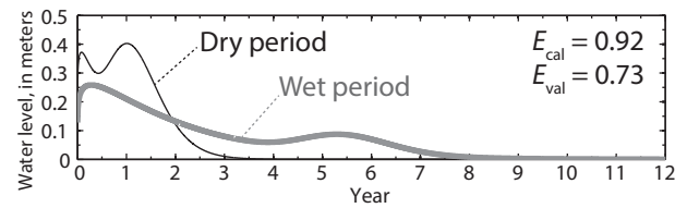
Figure 8. Example W1: impulse-response functions (IRFs) for well LA88C using double-gamma IRFs for both periods, i.e., wet and dry.
