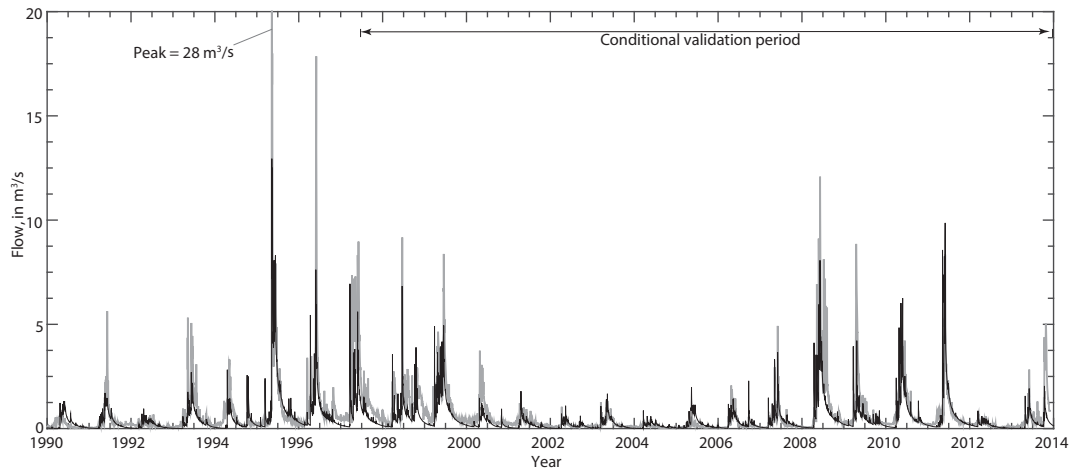
Figure 4. Example B3: observed (gray) and simulated (black) flow for Boxelder Creek.
