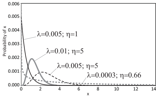
Figure 2. Gamma functions for different values of the two shape parameters.
