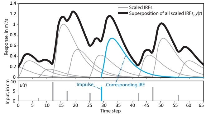
Figure 1. Superposition of sequential impulse-response functions (IRFs). Each IRF is in response to an impulse of the input function u_j and is scaled by the magnitude of that impulse.
