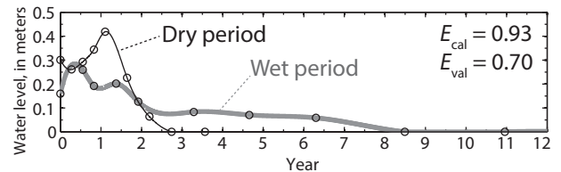
Figure 9. Example W2: nonparametric impulse-response functions for well LA88C using a total of 18 control points.
