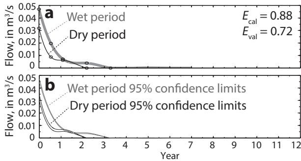
Figure 6. Example F8: nonparametric impulse-response functions (IRFs) for Barton Springs using a total of seven control points showing (a) optimized IRFs and (b) upper and lower 95 % confidence limits for the IRFs.
