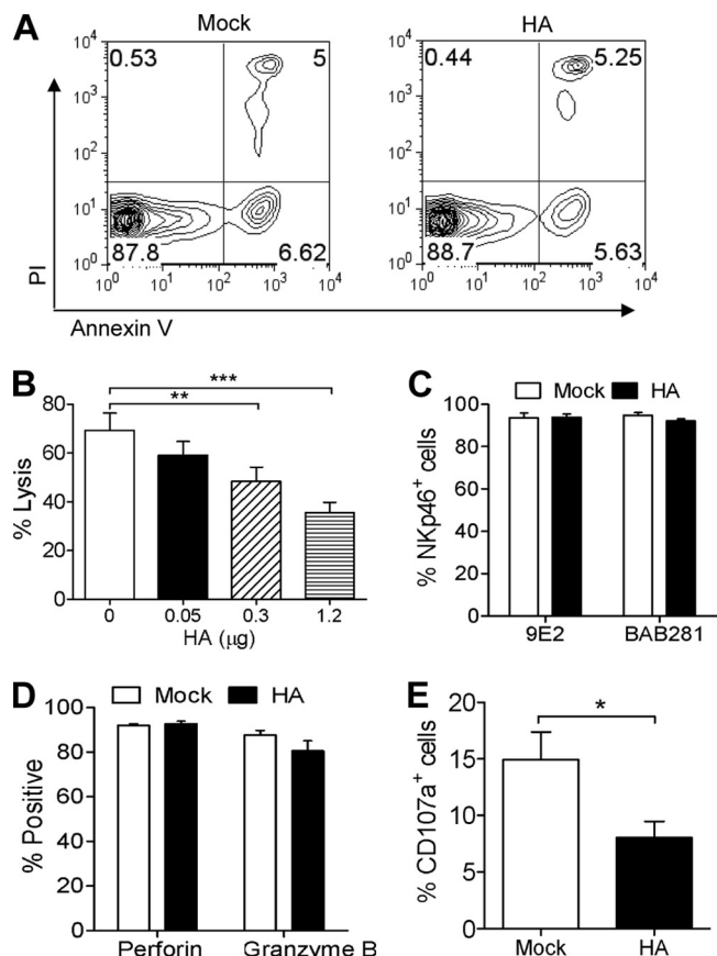
FIG. 4. Influenza virus HA inhibits granule exocytosis of NK cells upon target cell stimulation. (A) After either being left untreated or treated with 1 µg/ml influenza virus HA for 24 h, NK cells were examined by flow cytometry for annexin V binding and PI uptake. (B) Six-well plates precoated with HA protein were incubated with NK cells for 24 h. Cells were collected and examined for cytotoxicity against K562 cells at an E/T ratio of 20:1. Samples were analyzed by flow cytometry for the percentage of specific lysis. (C to E) Primary NK cells were treated with 1 µg/ml HA or left untreated (Mock) for 24 h. The cells were examined for the expression of surface NKp46 with two antibody clones, 9E2 and BAB281 (C), and of intracellular perforin and granzyme B (D) by flow cytometry. (E) The treated NK cells were collected and cocultured with K562 cells in the presence of anti-CD107a antibody for 2 h. The surface expression of CD107a on NK cells then was analyzed by flow cytometry. The data shown are means ± SEM from four different donors. *, P < 0.05 ; **, P < 0.01 ; ***, P < 0.001 .
